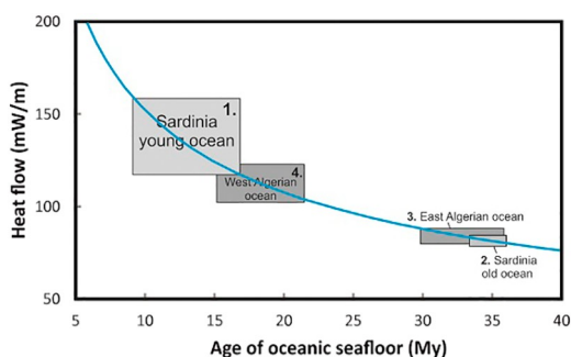
Fig. 8. A relation between the basement heat flow and the age of the oceanic seafloor can be considered in case a plate cooling model is valid in the region (Carlson and Johnson, 1994). For four selected regions of the oceanic part of the Western Mediterranean we plotted the mean heat flow and its standard variation on this graphic (see Fig. 7 for location of the regions). The resulting “apparent” ages are discussed in the text and compared with age estimates from geodynamic studies.
