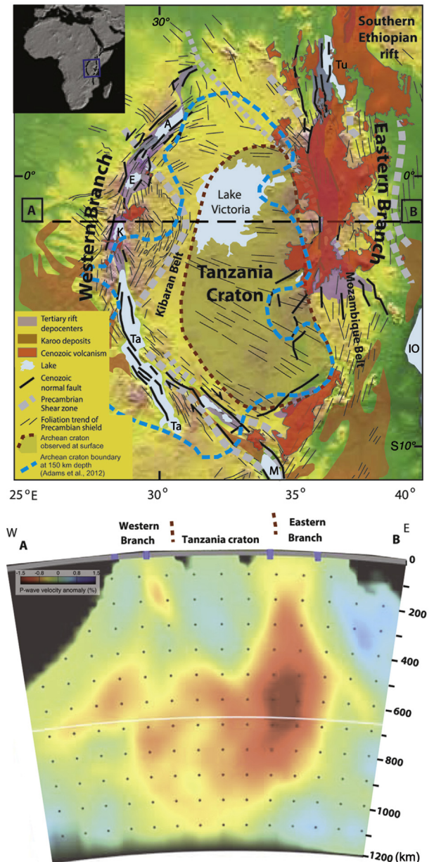
Figure 1. Geological and geophysical context. Top: Geological map of the EARS showing the surface extent of the Tanzanian craton, surrounded on both sides by active rift branches – the magma-poor western rift characterized by low-volume volcanic activity, large ( M > 6.5 ) magnitude earthquakes, and hypocenters at depths up to 30–40 km, while the magma-rich eastern rift is characterized by a broad zone of shallow (5–15 km) and smaller magnitude seismicity, but voluminous Cenozoic volcanism. Note the geometry (dashed line) of the craton boundary at 150 km depth (Adams et al., 2012). Bottom: E–W cross-section showing P-wave velocity mantle tomography observations (Mulibo and Nyblade, 2013a) that illustrate the thick Tanzanian craton underlain by hot mantle material deflected towards the eastern rift branch.
