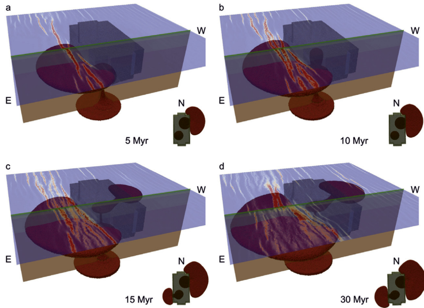
Figure 5. Model with 2 mantle plumes (Model 11, Table 1).
