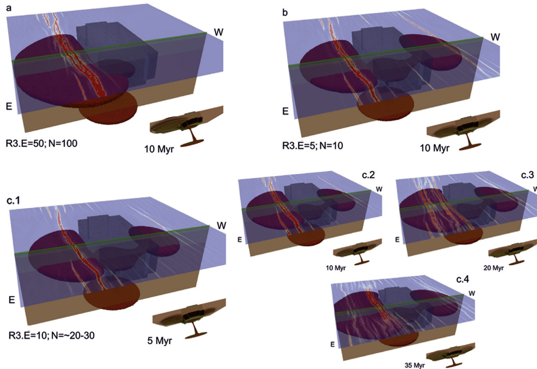
Figure 6. Models with small NE shifts of initial position of bigger ( r = 250 km) mantle plume (Models 18–20, Table 1).
