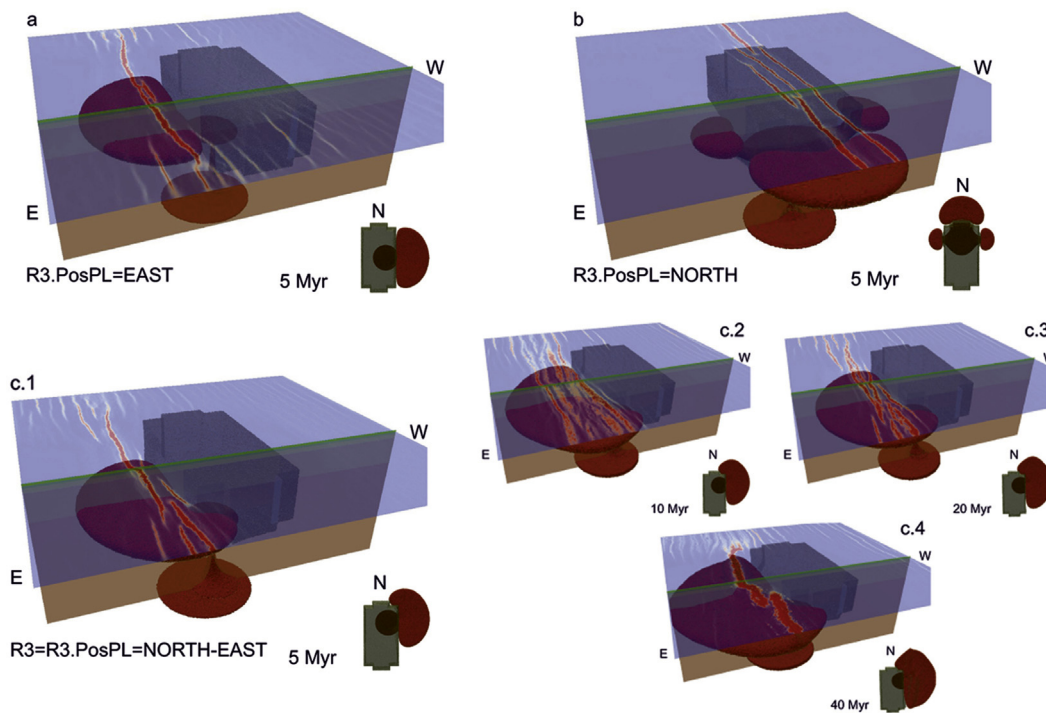
Figure 4. Models with different initial position of mantle plume with respect to craton (Models 2–4, Table 1).
