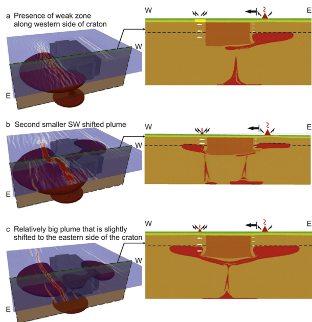
Figure 9. Three possible scenarios explaining main EARS features. (a) The assumption of rheologically weak interface along the western border of the craton (Model 7); (b) the presence of second smaller plume initially shifted in SW direction (Model 11); (c) the unequal splitting of relatively big plume which initial position is slightly shifted to the eastern side of the craton (Model 20).
