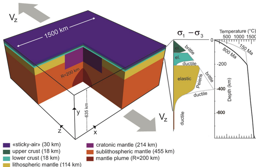
Figure 2. Model setup. Gray arrows show the velocity boundary conditions, applied in a direction perpendicular to the model domain. The initial radius of the plume is 200 km.
