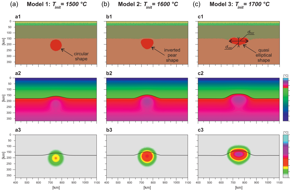
Figure 4. (a) Model 1 ( T_{init} : 1500 °C; *); (b) model 2 ( T_{init} : 1600 °C; *) and (c) model 3 ( T_{init} : 1700 °C; *) represented by (1) material phase field (upper row); (2) distribution of the temperatures ( T ; middle row); (3) temperature contrasts ( \Delta T ; lower row) at the time slice of 60 Myr. *Other experimental parameters: d_{init} : 100 km; type of lithosphere: ‘Variscan’; V_{ext} : 0 mm \times yr ^{-1} .
