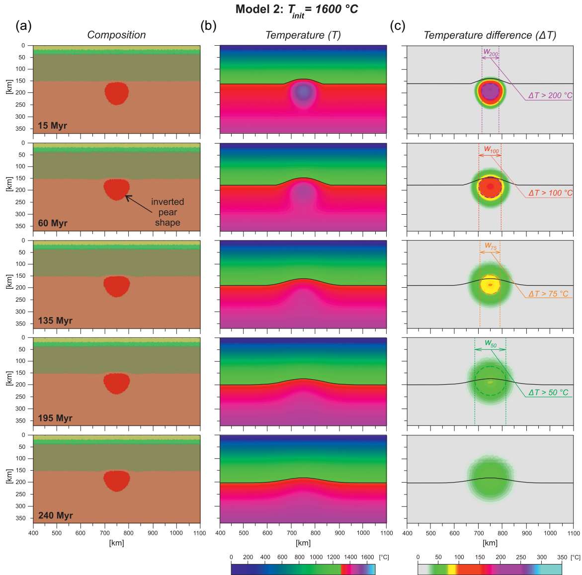
Figure 3. Temporal evolution of model 2 ( T_{init} : 1600\text{ }^{\circ}\text{C} ; d_{init} : 100\text{ km} ; type of lithosphere: ‘Variscan’; V_{ext} : 0\text{ mm} \times \text{yr}^{-1} ): (a) material phase field. Since 60 Myr the plume has an inverted pear (or a light bulb) shape; (b) distribution of the temperatures ( T ) and (c) temperature contrasts ( \Delta T ). The areas A_x and corresponding w_x are shown in the panel ‘c’ for the following \Delta T thresholds: x = 200, 100, 75 and 50\text{ }^{\circ}\text{C} .
