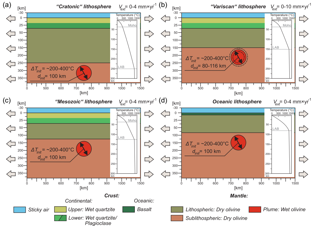
Figure 2. Design of 2-D model setup for four tested types of lithosphere: (a–c) Continental lithosphere: (a) ‘Cratonic’, (b) ‘Variscan’, (c) ‘Mesozoic’ and (d) oceanic lithosphere ( \sim 40 Ma old). Insets show the initial temperature distributions. A circular-shaped mantle plume anomaly is seeded just below the bottom of the lithosphere. Lateral velocities ( V_{\text{ext}} ) are applied at vertical sides of the model.
