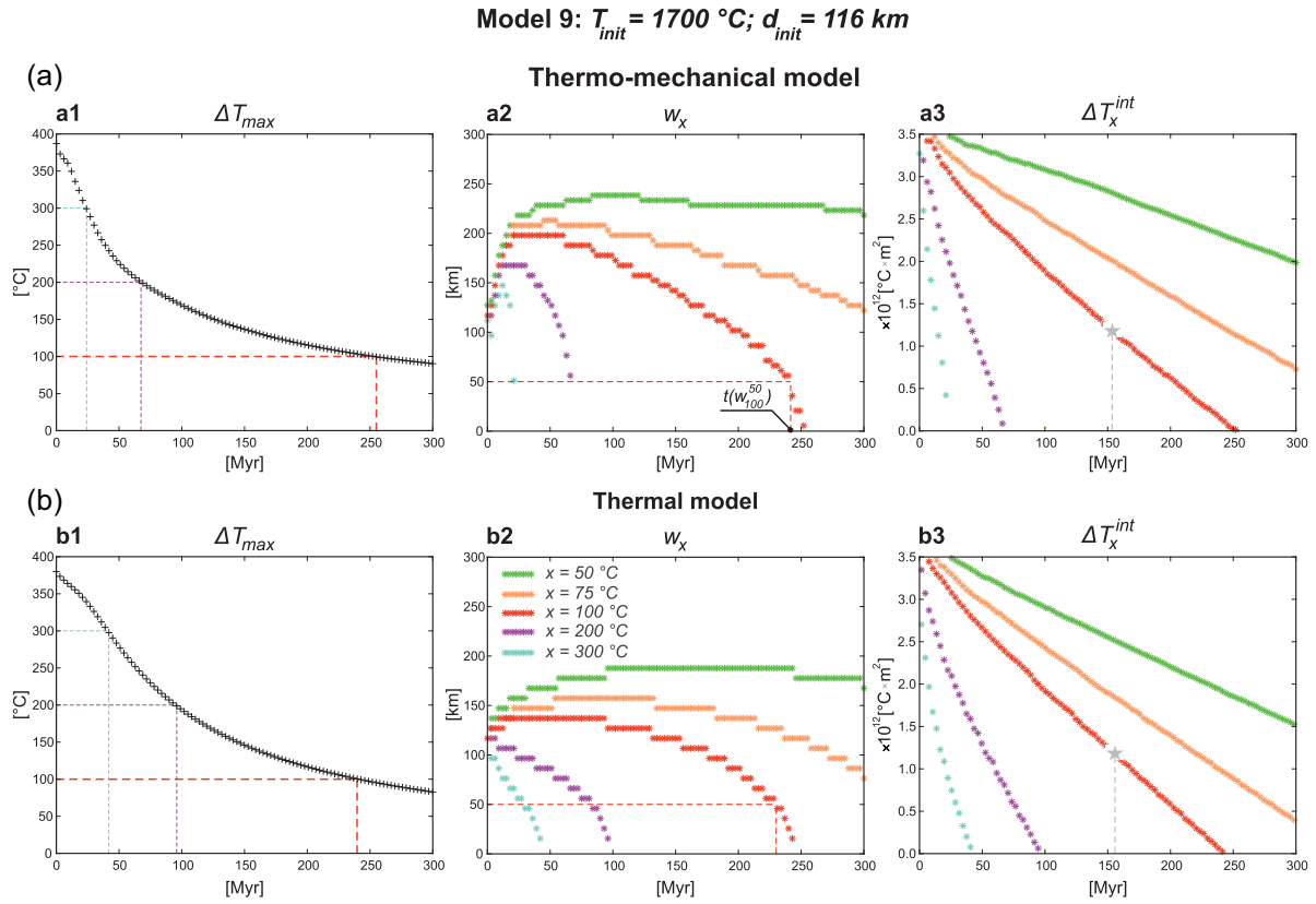
Figure 8. Temporal evolution of model 9 ( T_{init} : 1700\text{ }^{\circ}\text{C} ; d_{init} : 116\text{ km} ; type of lithosphere: ‘Variscan’; V_{ext} : 0\text{ mm} \times \text{yr}^{-1} ) for (a) thermomechanical and (b) thermal versions represented by parameters derived from \Delta T . Figure conventions as in Fig. 5.
