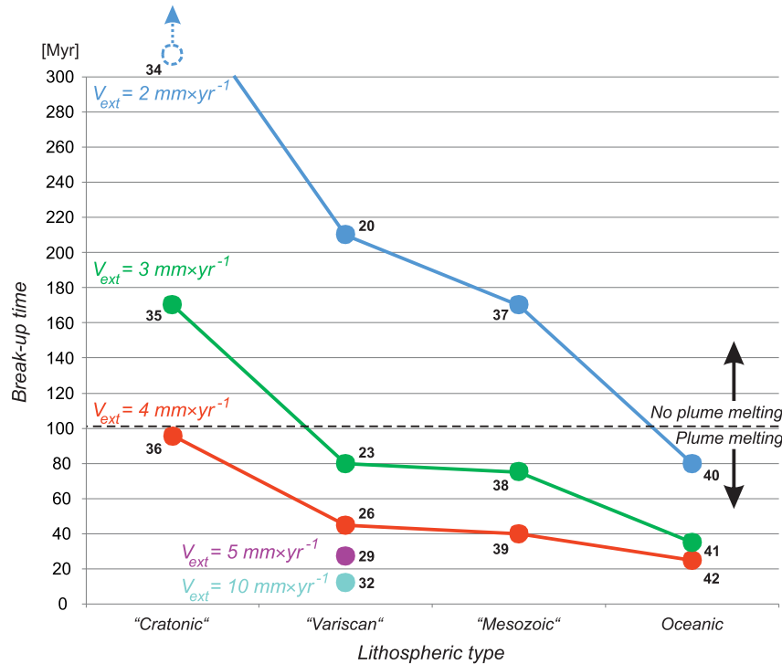
Figure 16. Models 20, 23, 26, 29, 32, 34–42 ( T_{init} : 1600 °C; type of lithosphere: ‘Cratonic’, ‘Variscan’, ‘Mesozoic’, oceanic; V_{ext} : 2–10 mm \times yr ^{-1} ; d_{init} : 100 km): break-up time as a function of lithospheric type. Blue, green and red lines correspond to V_{ext} of 2, 3 and 4 mm \times yr ^{-1} , respectively. Magenta and aqua colours refer to the models of ‘Variscan’ lithosphere with V_{ext} of 5 and 10 mm \times yr ^{-1} . The numbers of the models are labelled.
