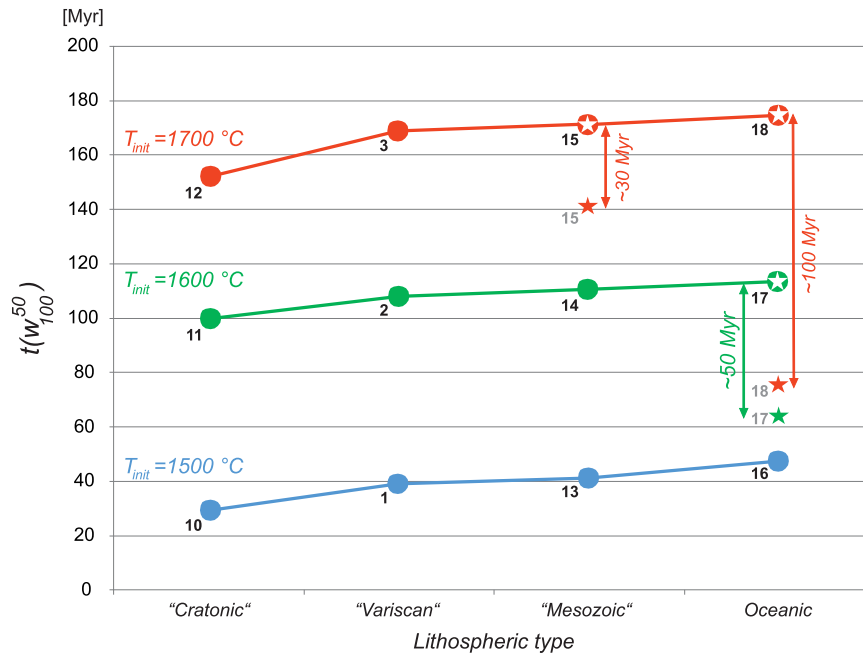
Figure 12. Models 1–3, 10–18 ( T_{init} : 1500–1700 °C; type of lithosphere: ‘Cratonic’, ‘Variscan’, ‘Mesozoic’ and oceanic; d_{init} : 100 km; V_{ext} : 0 mm \times yr ^{-1} ); plume lifespan t(w_{100}^{50}) as a function of lithospheric type. Blue, green and red colours correspond to T_{init} of 1500, 1600 and 1700 °C, respectively. The numbers of the models are labelled. Other figure conventions as in Fig. 9.
