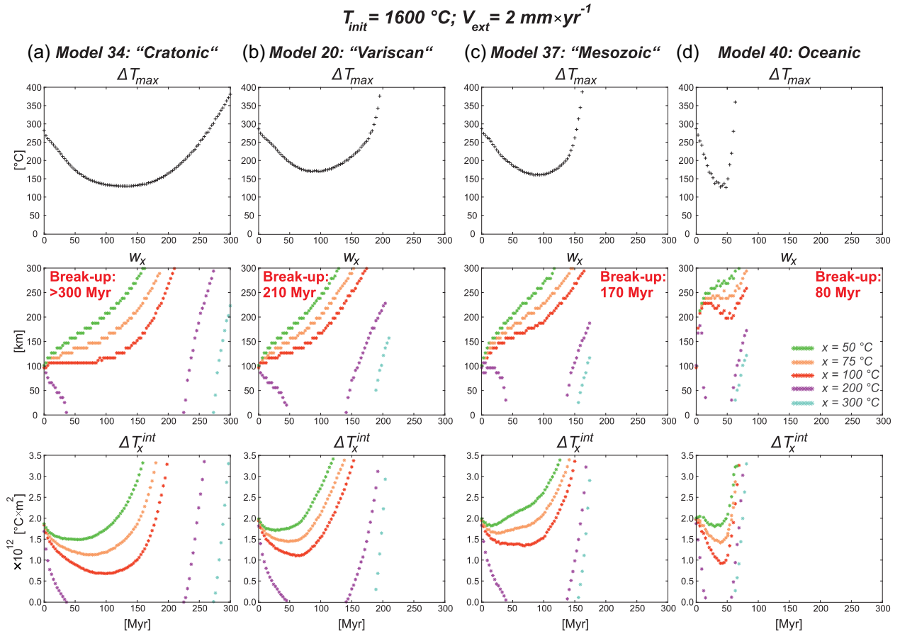
Figure 15. Temporal evolution of the experiments characterized by T_{init} of 1600 \text{ }^\circ\text{C} , V_{ext} of 2 \text{ mm} \times \text{yr}^{-1} and different types of lithosphere: (a) model 34 ('Cratonic' lithosphere; d_{init} : 100 km); (b) model 20 ('Variscan' lithosphere; d_{init} : 100 km); (c) model 37 ('Mesozoic' lithosphere; d_{init} : 100 km) and (d) model 40 (oceanic lithosphere; d_{init} : 100 km) represented via parameters derived from \Delta T . Figure conventions as in Fig. 5.
